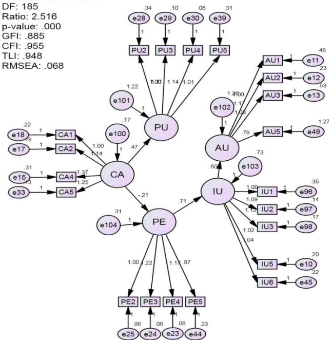
Figure 6. Final Model
