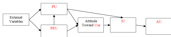
Figure 1. TAM
