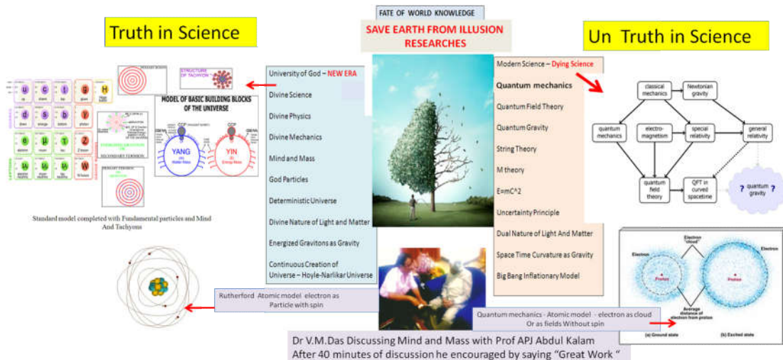
Fig 19 If Spin of particles collapses the entire universe effects(structural effects, physical effects, chemical effects and spectral effects), life sciences effects would be collapsed
