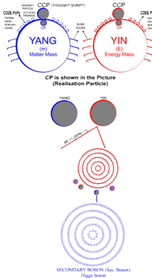
Fig. 19. Structure of Higg's Bosons
