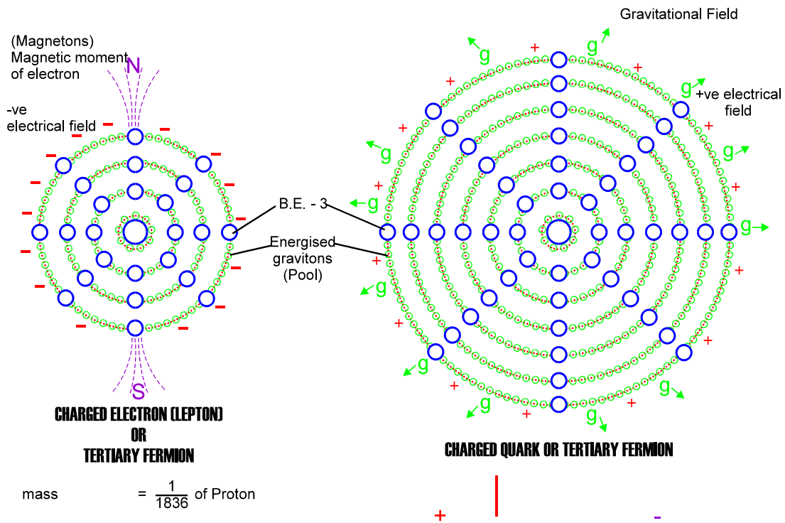
Fig. 25. Structure of Leptons and Quarks
