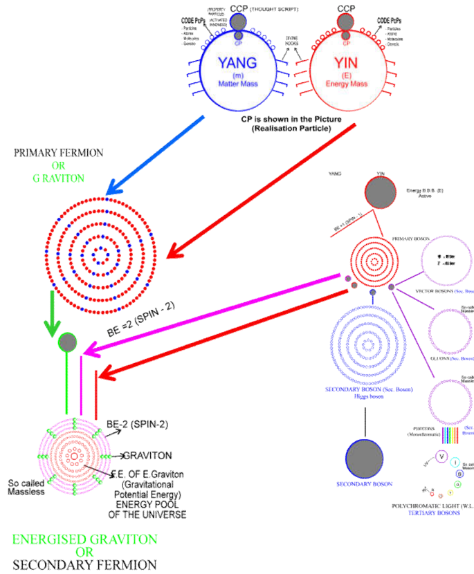
Fig. 18. Structure of Gravitons and Energized Gravitons
