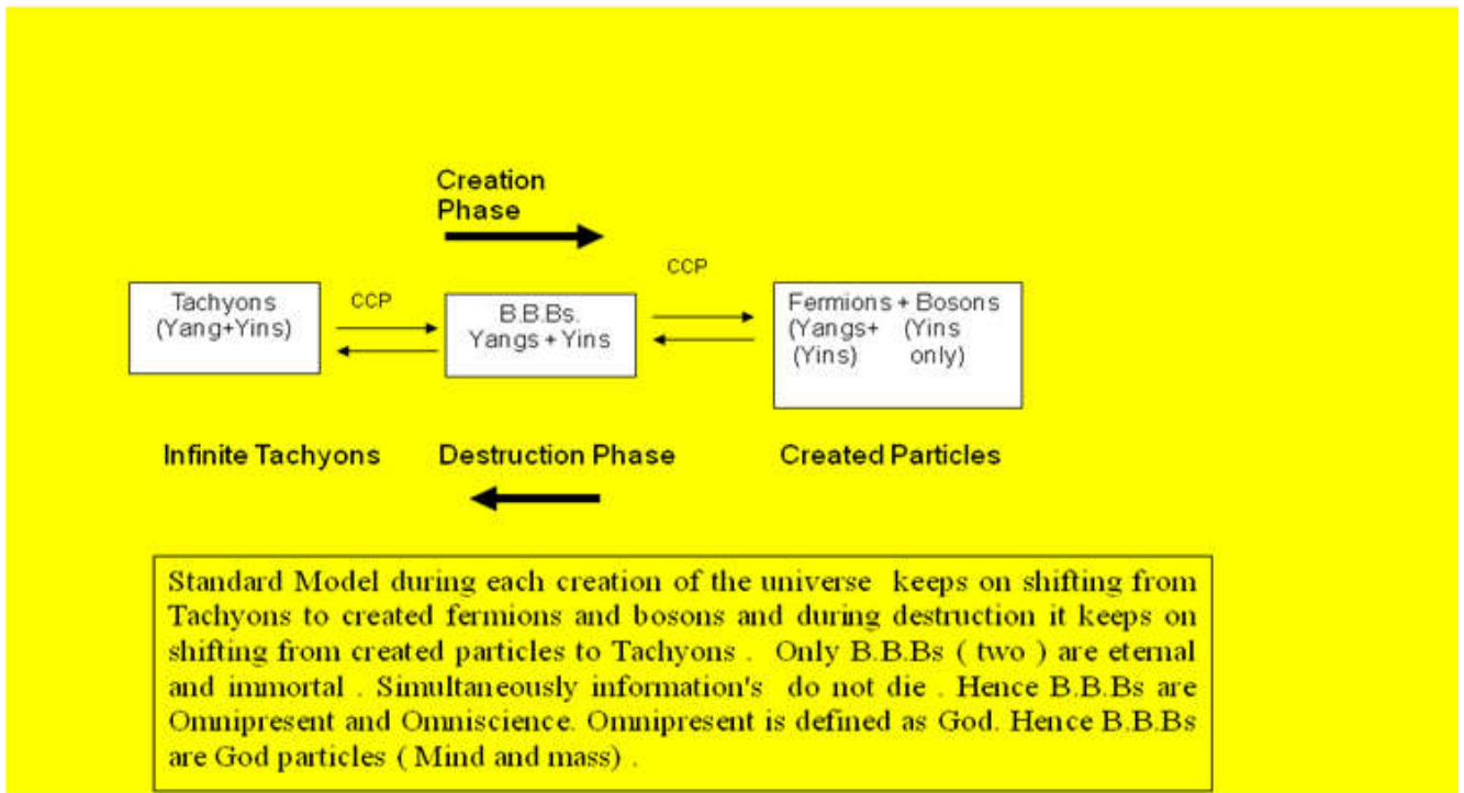
Fig. 40. Symmetry and Symmetry breaking Phases at the time of Origin of Universe
