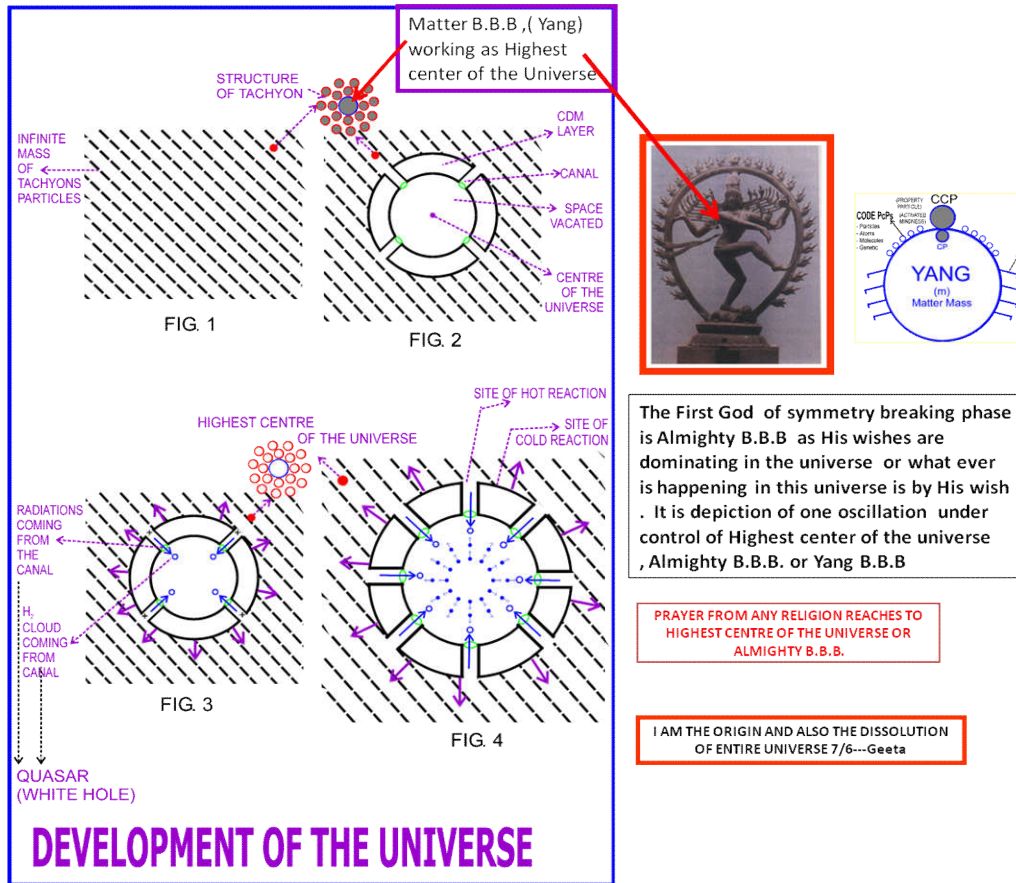
Fig. 28. Hoyle Narlikar Universe OR Universe "I"
