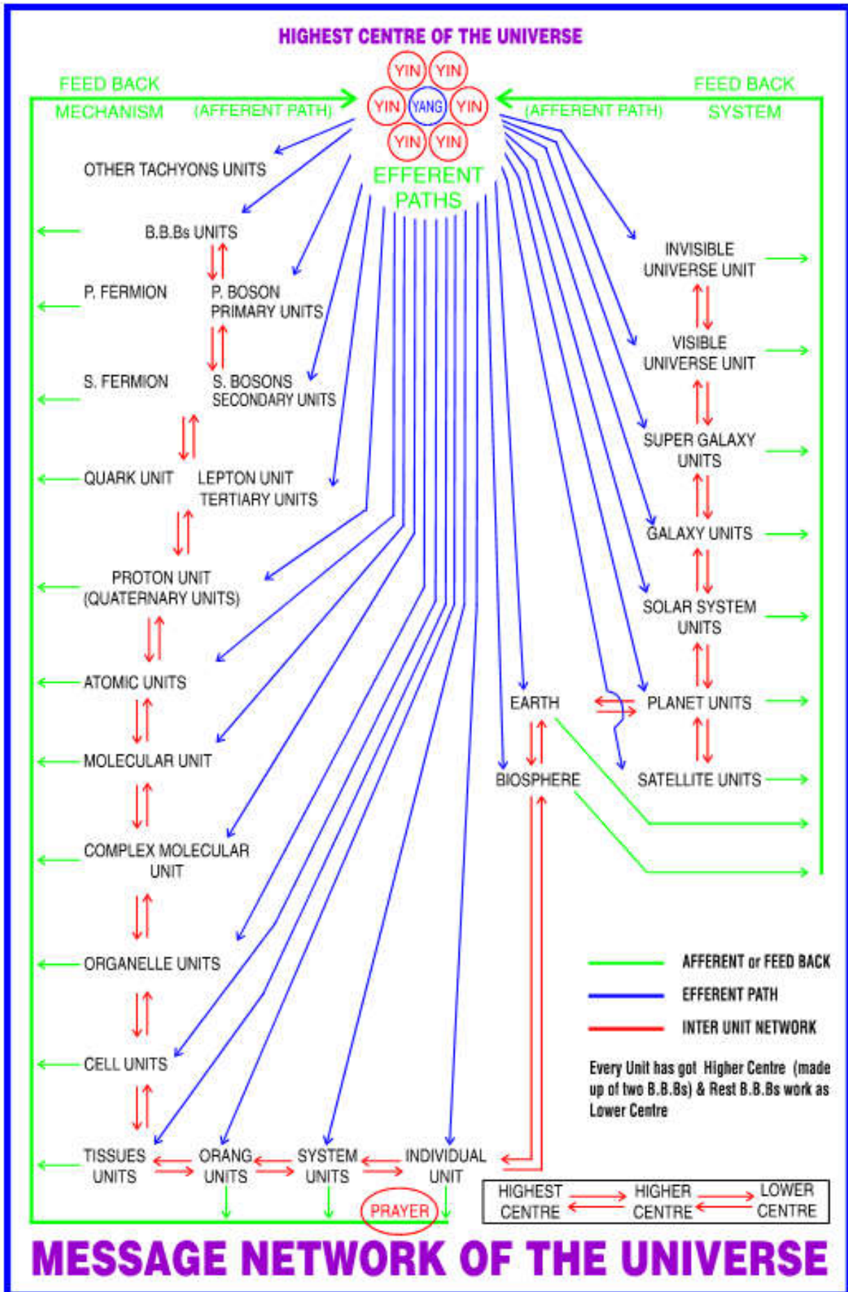
Fig. 17. Feed back Mechanism by Quantum Entanglement (1 st atomic transcription)
