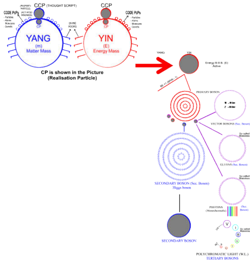
Fig. 7. Structure of Bosons Completed
