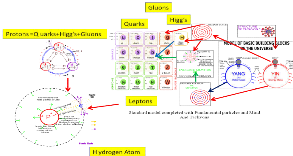
Fig. 34. Standard Model Chart modified and completed
