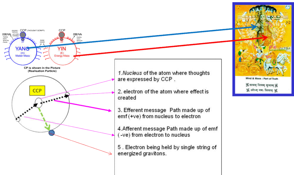
Fig. 26. Working of hydrogen atom – Divine MONB Theory
