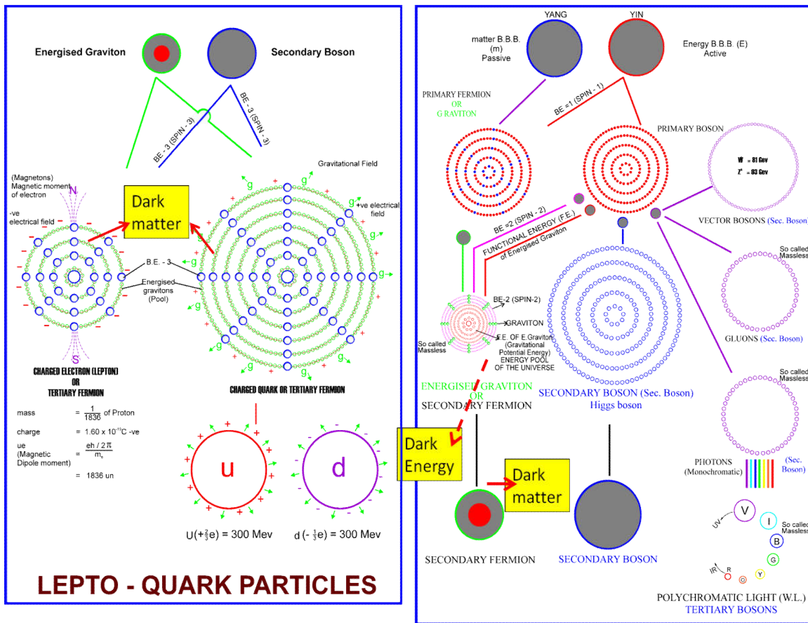
Fig. 13. Dark Matter and Dark Energy at micro level
