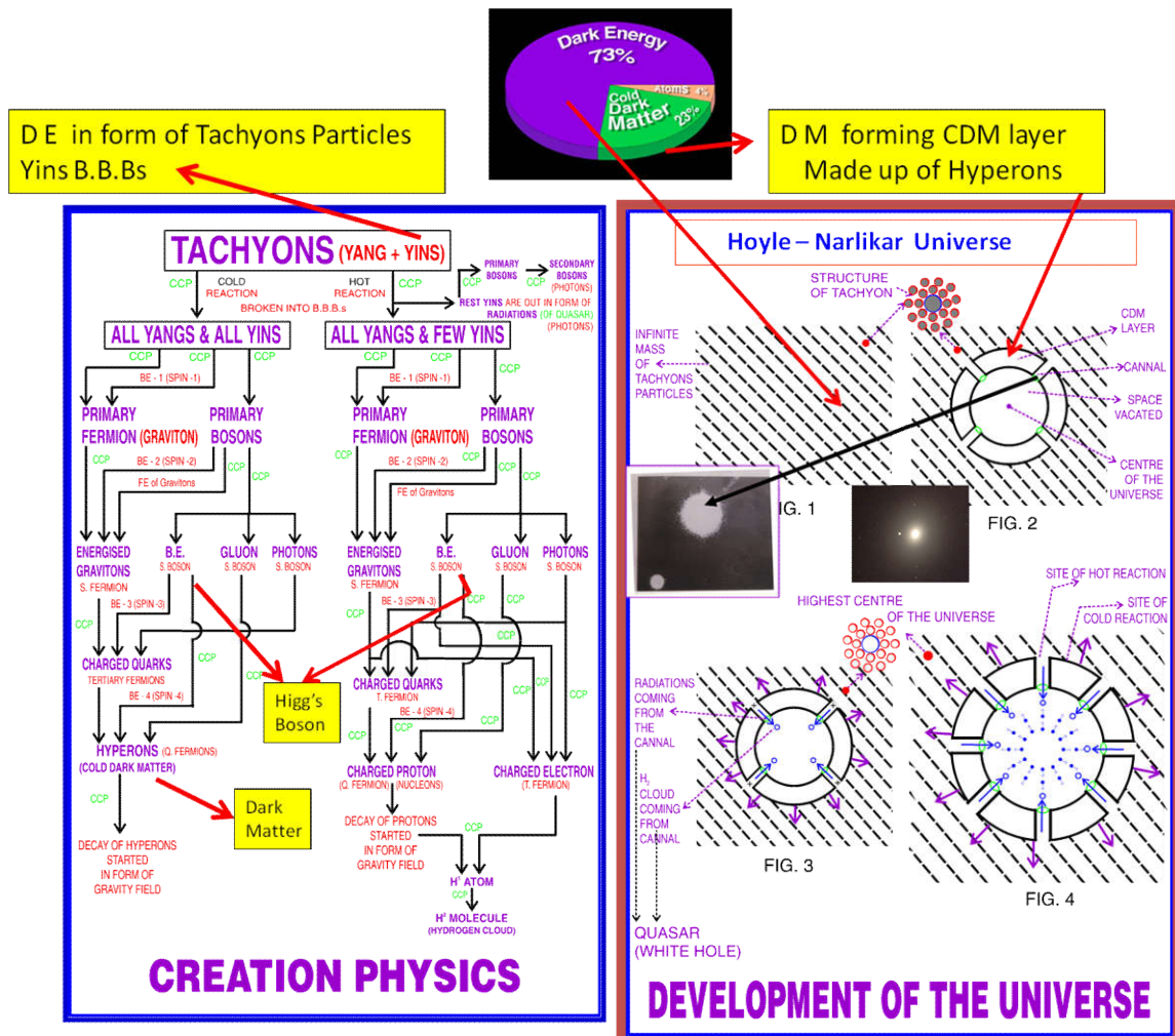
Fig. 12. Dark matter and Dark Energy at macro level
