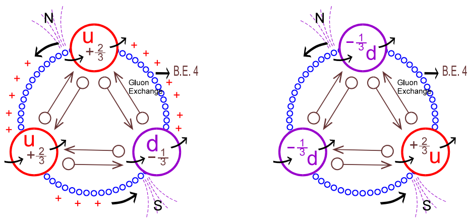
Fig. 33. Complete Structure of Proton and structure of Neutron
