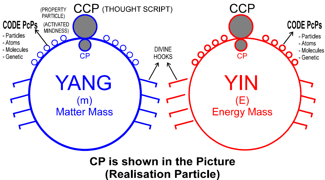
Fig. 43. Primary God or “I” or Basic Building Blocks or Yang and Yin
