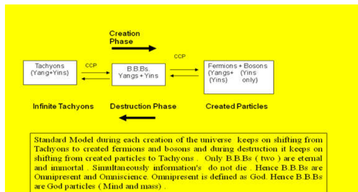
Fig. 3.1. One creation and destruction cycle [4]
