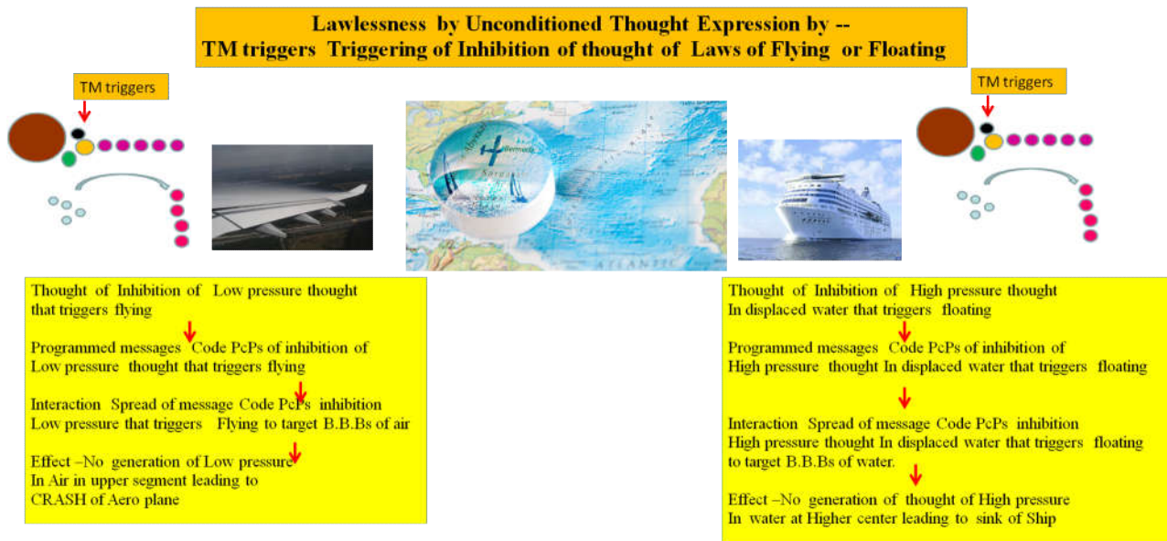
Fig. 22. Phenomenon of Lawlessness triggered by unconditioned thought expression by Time mindness that led to inhibition of thought of law of Floating Or Flying in Bermuda triangle leading to sinking of ship or crashing of aero plane (macro level)
