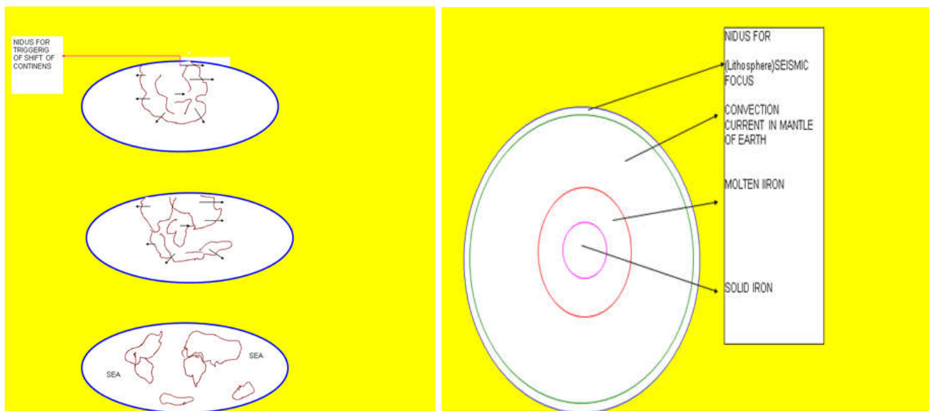
Figure 16. Shifting of continents Figure 17. Nidus for seismic foci
