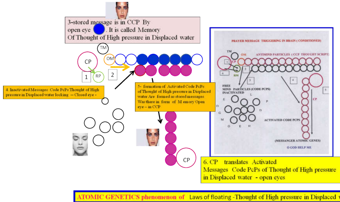
Fig. 18. Triggering of Law of Floating thought of High pressure in displaced water (micro level)
