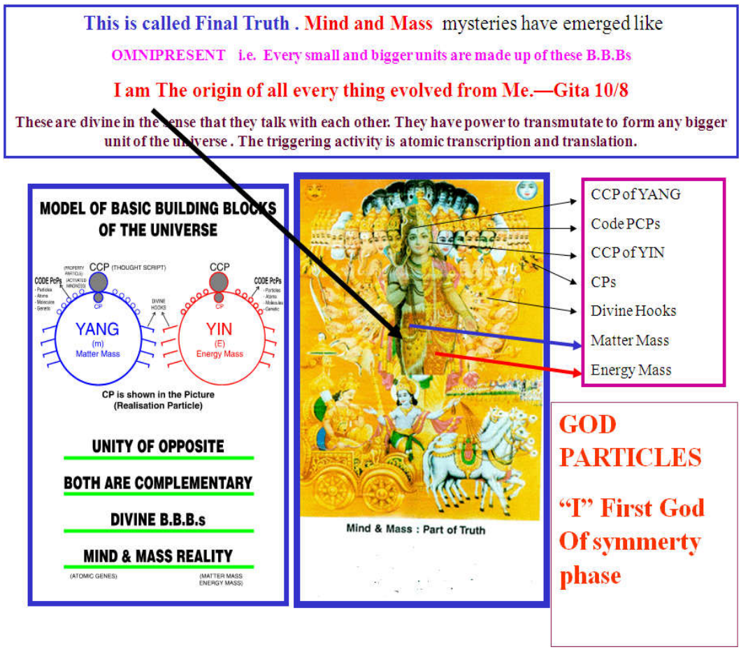
Fig. 1. Divine Mechanics Unit – CCP, CP and information s – Code PcPs with B-Bit – Mass
