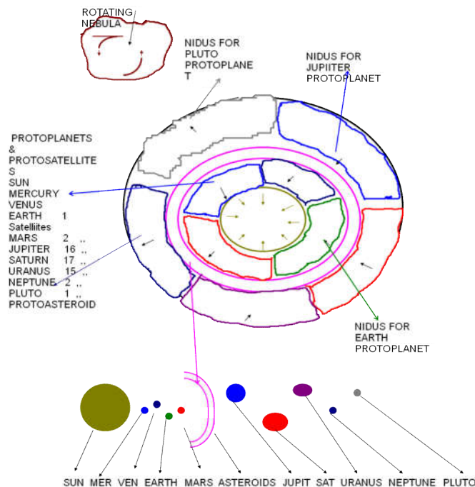
Figure 15. Origin of solar system
