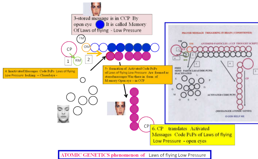
Fig. 19. Thoughts of Law of Flying Triggering of thought of Bernoulli's principle Low pressure Code PcPs (micro level)
