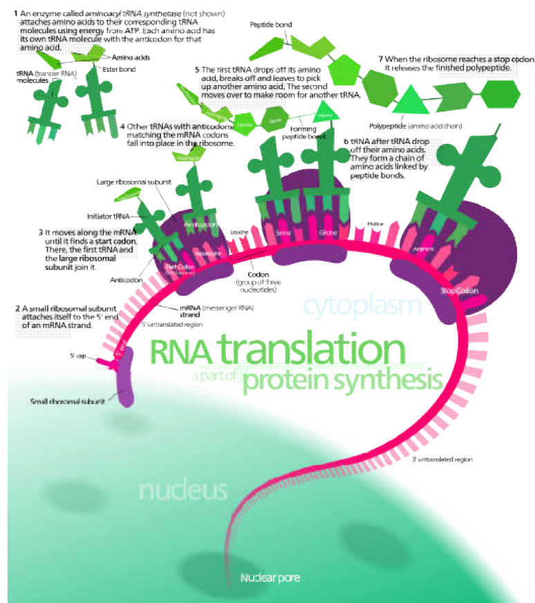
Diagram showing the process of translation
